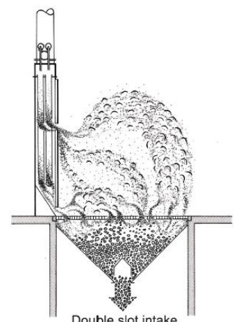
Double slot intake.
